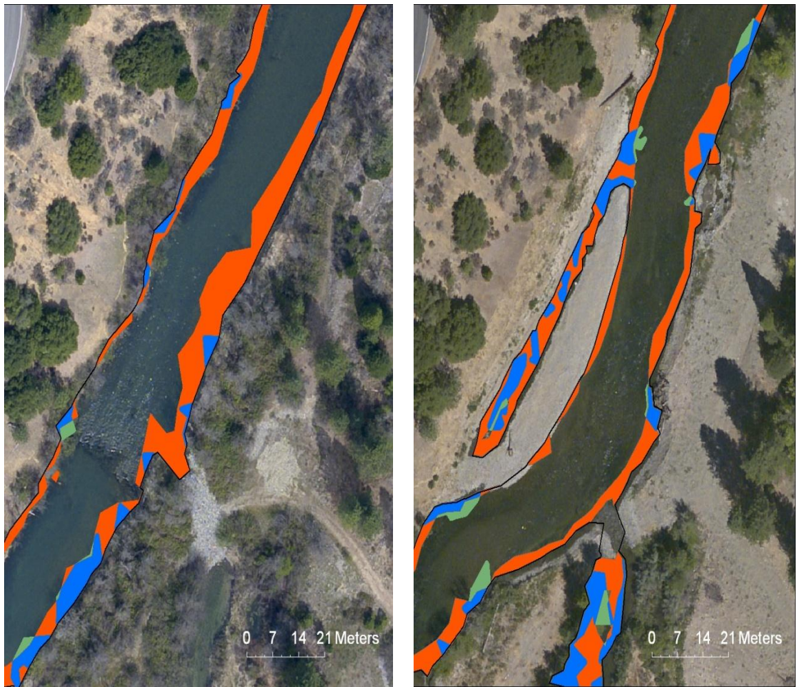
Figure 10. Aerial views of forced meander location at Sawmill rehabilitation site (rkm 176.0) before construction (left photo) and after construction (right photo). Black lines indicate the wetted edge, blue areas indicate optimal presmolt habitat and red and green areas indicate suitable presmolt habitat. Mainstem discharge pre-construction was 8.3 cms (294 cfs) and 8.5 cms (304 cfs) post-construction.
