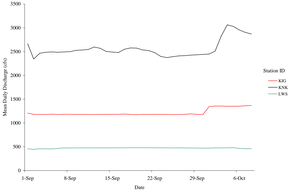
Figure 1. Mean daily discharge (cfs) of the Klamath and Trinity rivers during the adult Chinook salmon pathology monitoring sampling period, September and October, 2005. Discharge was estimated on the Klamath River near Iron Gate Dam (KIG), near Klamath (KNK), and on the Trinity River near Lewiston (LWS).
